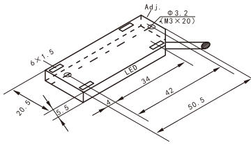
KCS 20.5 20.5x50.5x5.5
