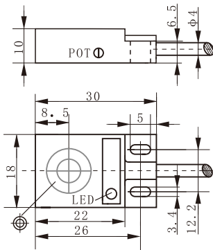
KCS 18 18x30x10
