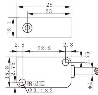
KCS 15.8 15.8x28x12.1
