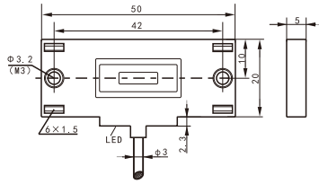
KCS 20 20x50x5
