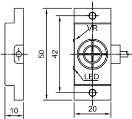
KCS 20 20x50x10
