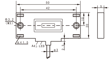
KCS 20 20x50x5
