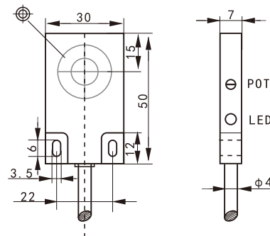
KCS 30 30x50x7
