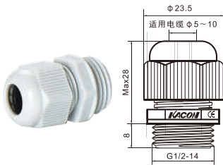
PG13.5A
